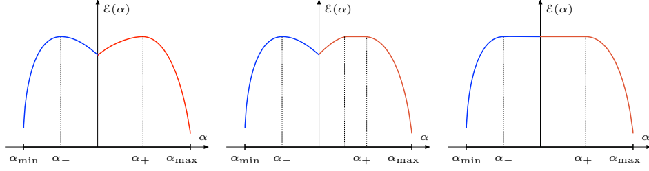
FIGURE 1. Possible shapes of entropies. Left figure: assuming proximality
