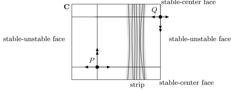
FIGURE 2. Blender-horseshoe: strong unstable curves and strips (projection along the strong stable direction)
